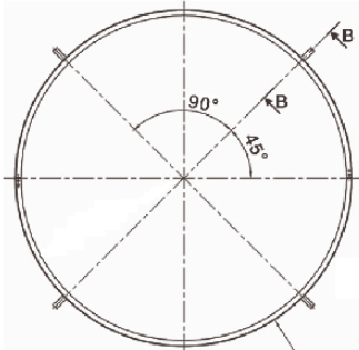
Winkel 35x35x4
